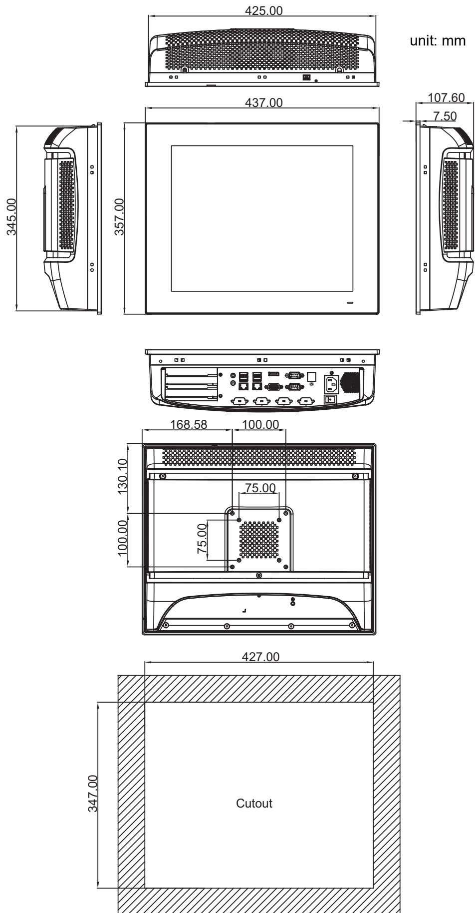
Figure 1.2 PPC-6171C Dimensions
