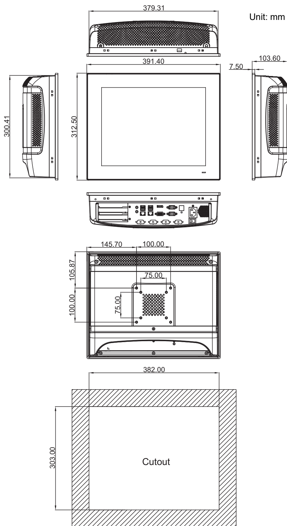
Figure 1.1 PPC-6151C Dimensions
