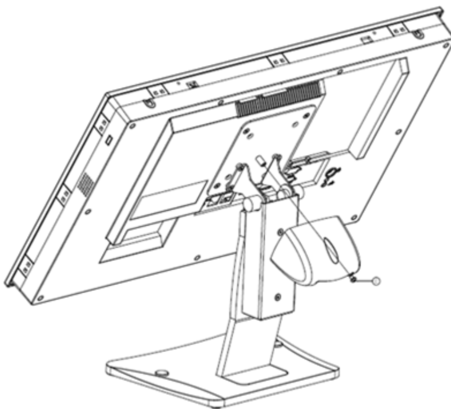
Figure 2.9 Securing the Stand Mount Hinge Cover
