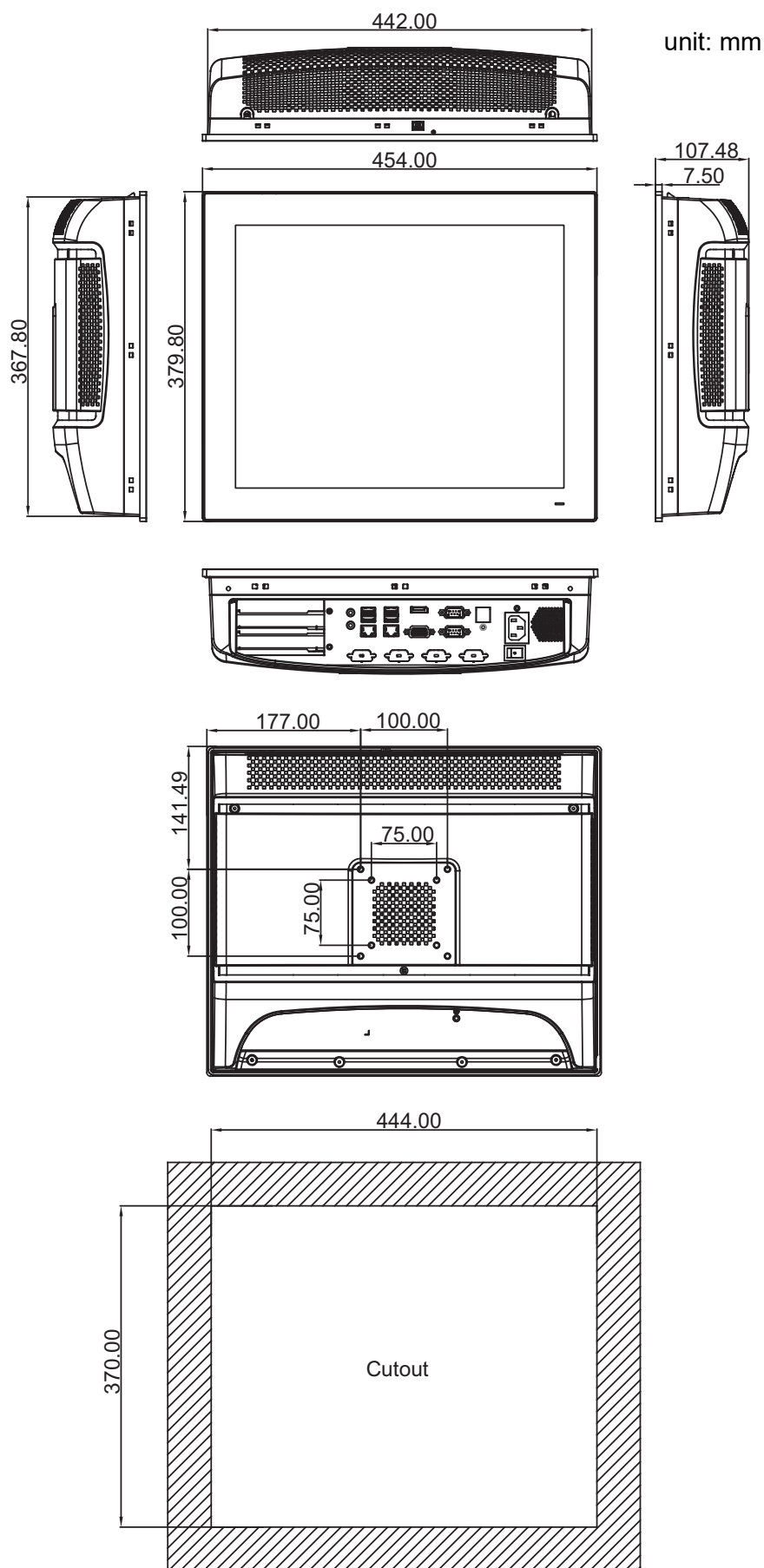
Figure 1.3 PPC-6191C Dimensions
