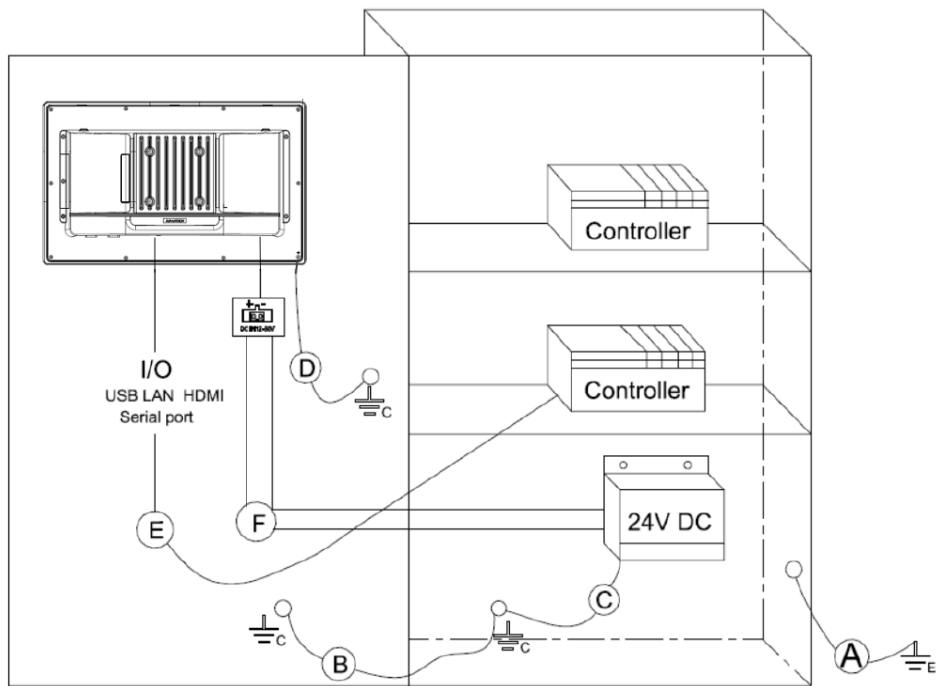
Figure 2.21 System Wiring
