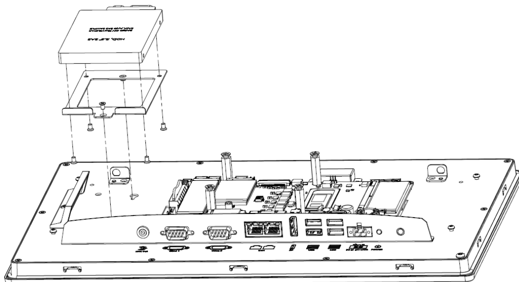
Figure 2.4 SSD Installation
